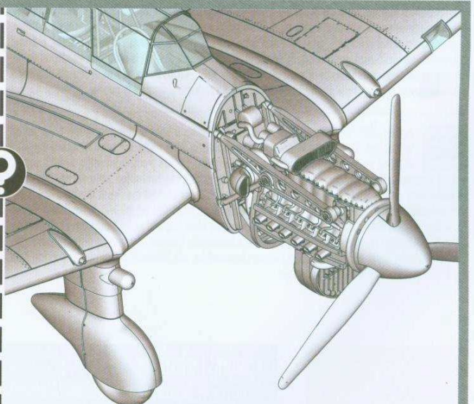
To build the model with the engine in place miss out steps 53 to 65.
