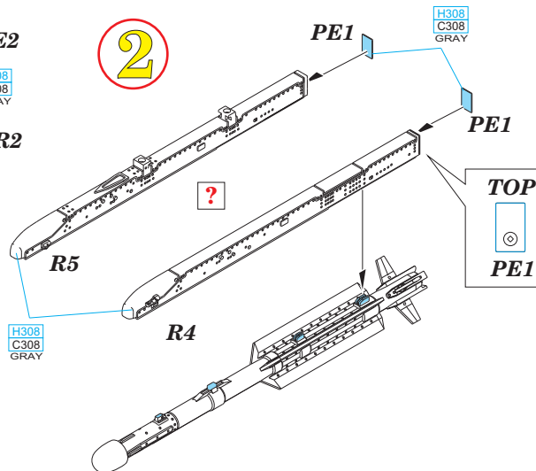
R5 - Lavett RB99 for JAS-39
