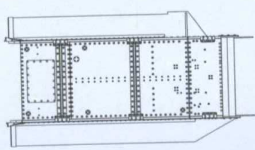
Lower Hull
