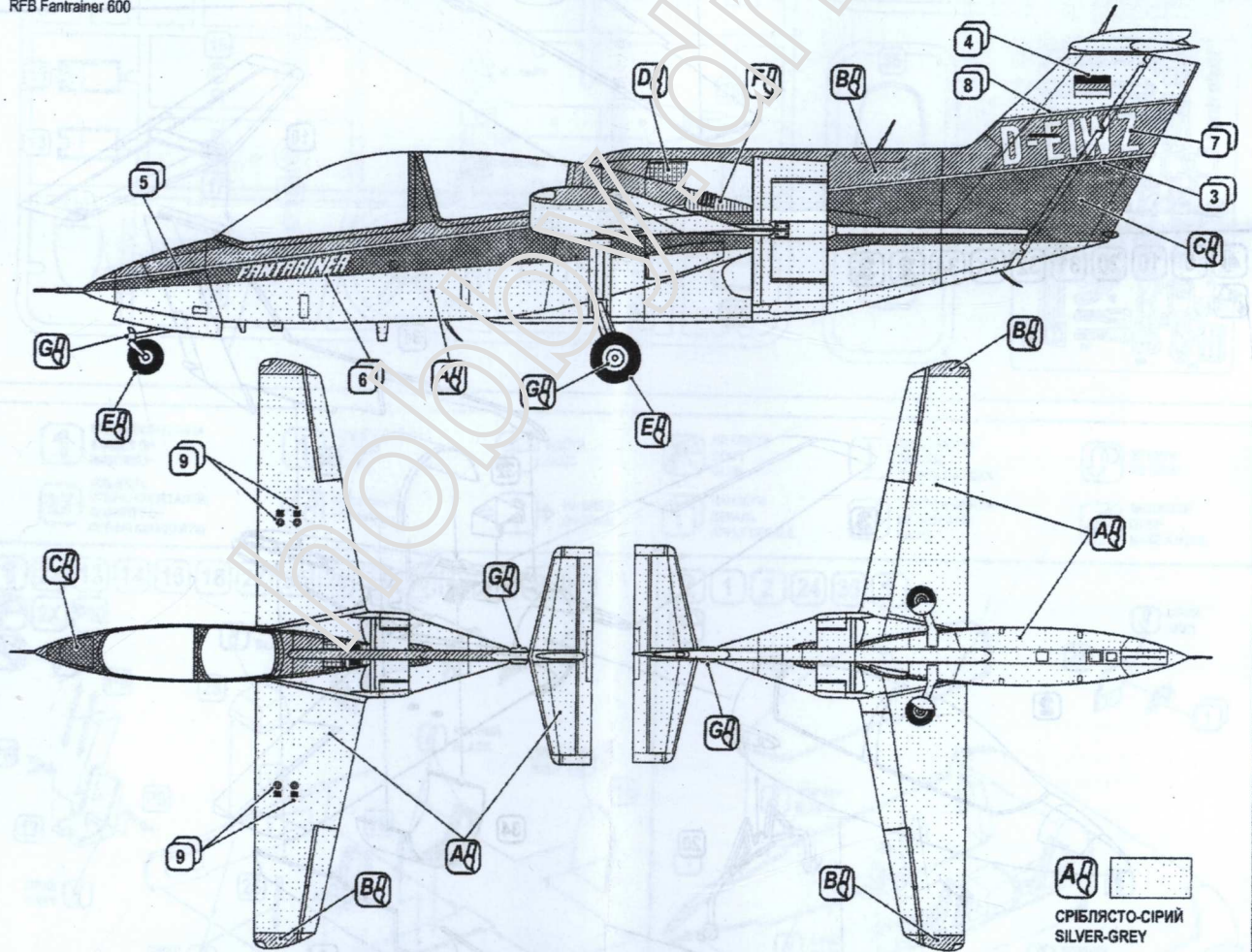
RFB Fantrainer 600
