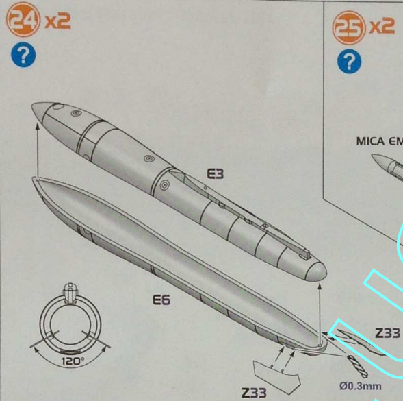
RP-541/542 2000L Fuel Tank
