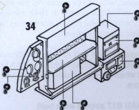
REAR INSTRUMENT PANEL
