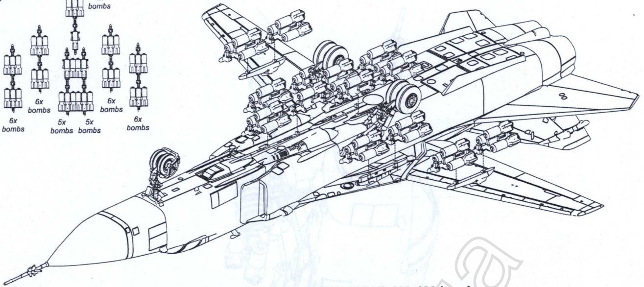
Su-24M bomber version w/ 38x OFAB-100-120 bombs
