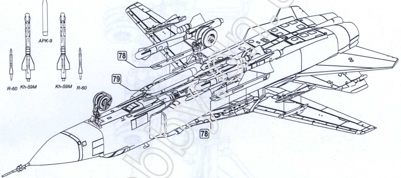
Su-24M missile carrier w/ 2x Kh-59 "Ovod" cruise missiles
