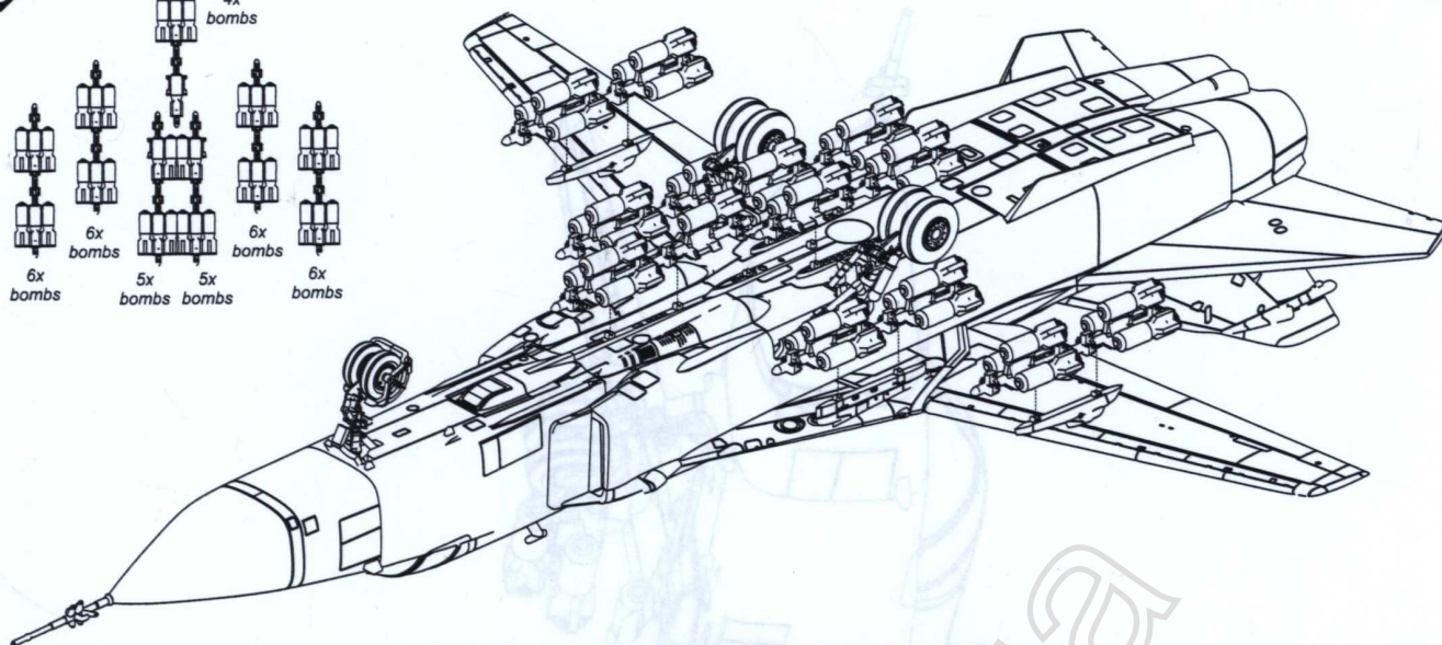
Su-24M bomber version w/ 38x OFAB-100-126 bombs
