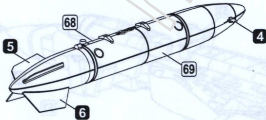
OFAB-100-120 bombs on MBDZ-U6-68 rack
