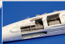
7452 F-14A Tomcat Port Side Cannon Installation
